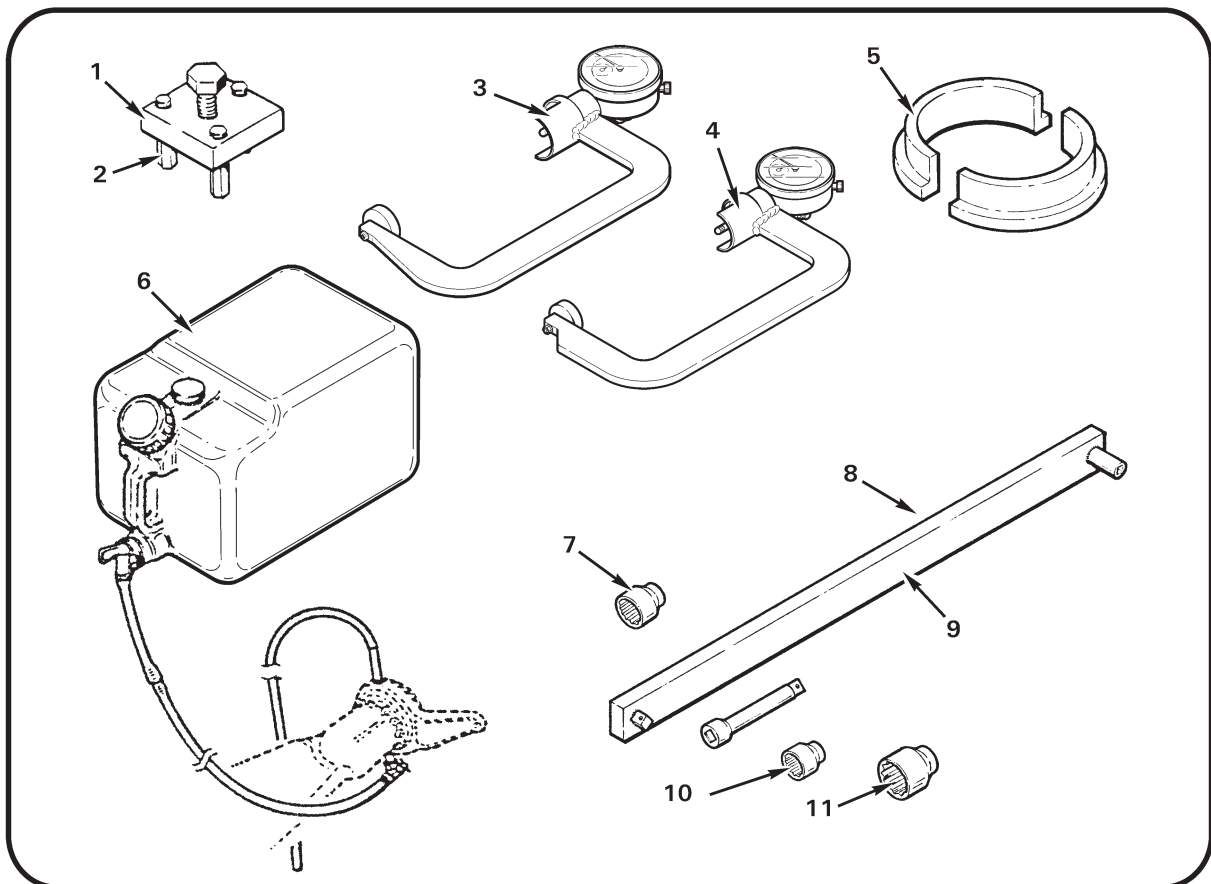
FIGURE 36-2 SPECIAL TOOLS
