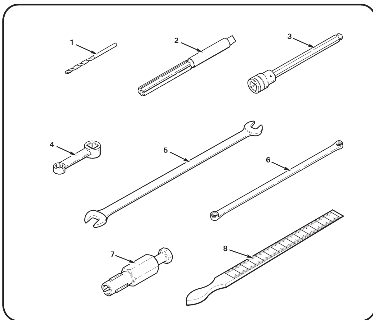
FIGURE 36-6 SPECIAL TOOLS
