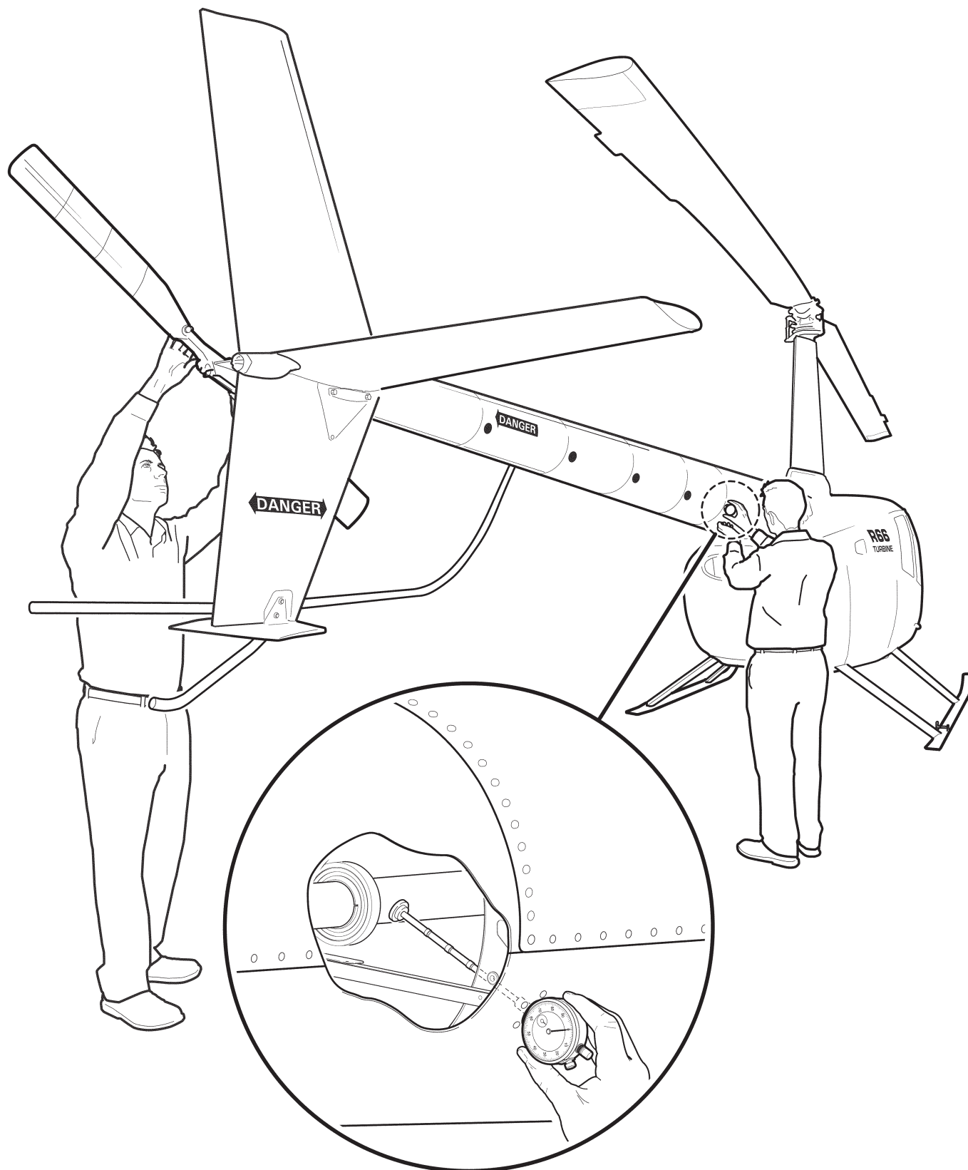
FIGURE 65-2 RUNOUT
